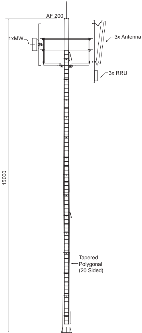
15M Monopole 1 Station
