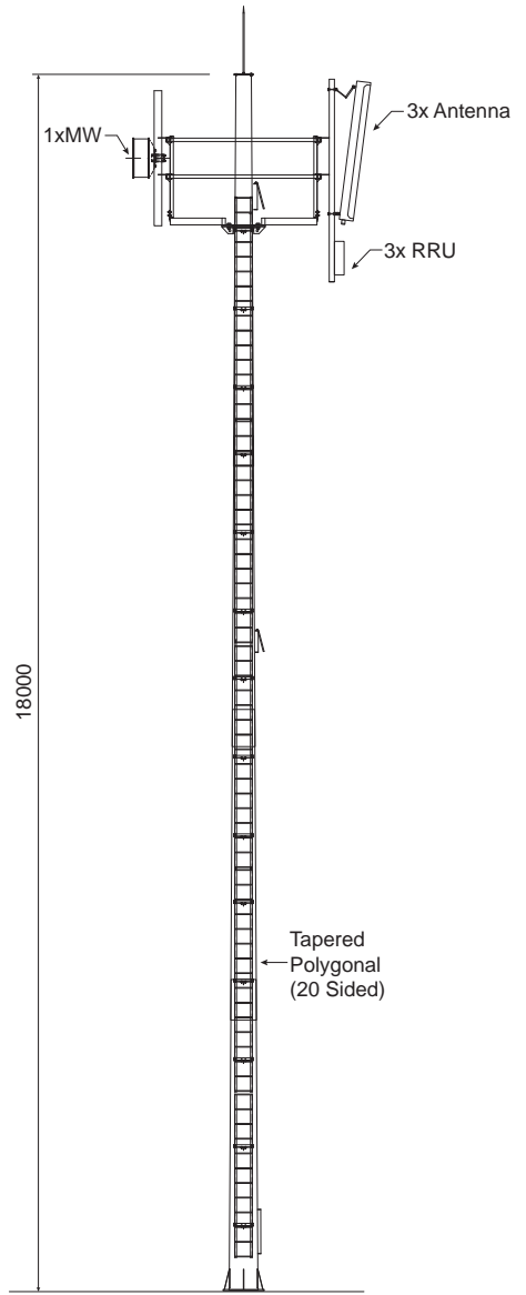
18M Monopole 1 Station
